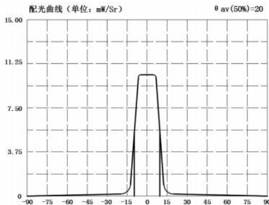
Fig.2- Light intensity distribution (Cartesian coordinates)-Y
