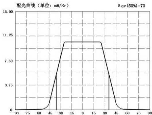
Fig.1- Light intensity distribution (Cartesian coordinates)-X
